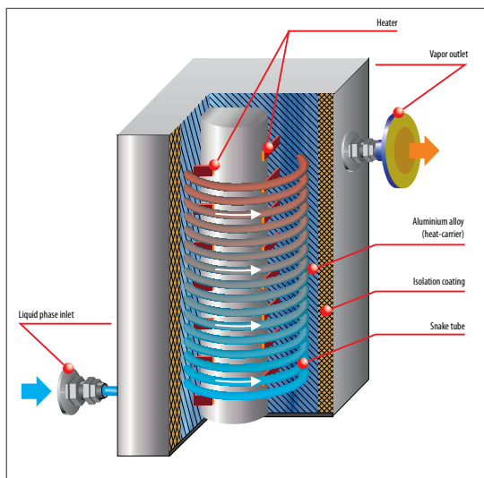
Operating diagram of dry type vaporizer EDS 2000
