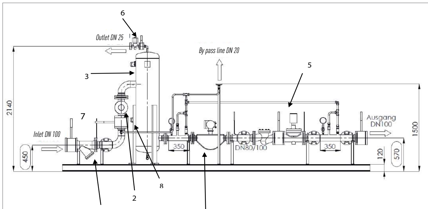
Drawing scheme EDS 93 1053 complete measuring line
