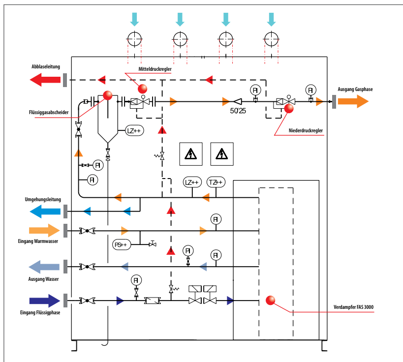
Hydraulic schema of vaporizer unit EDS 3000-200
