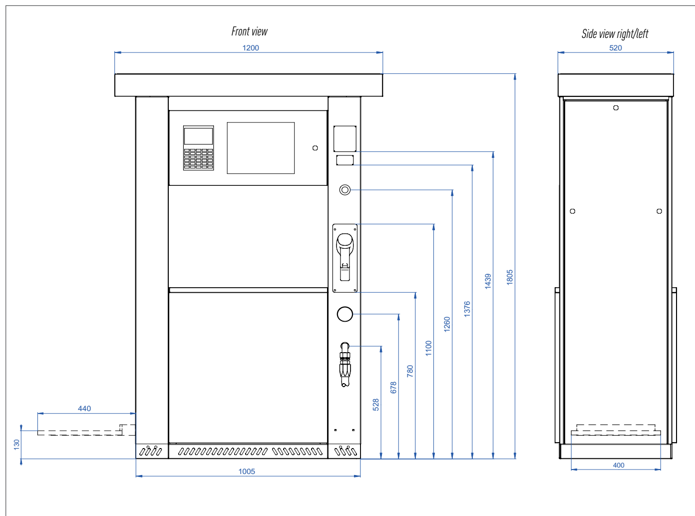
Dimensional drawing of electronic LPG-dispenser type EDS-220 WM with filling device
