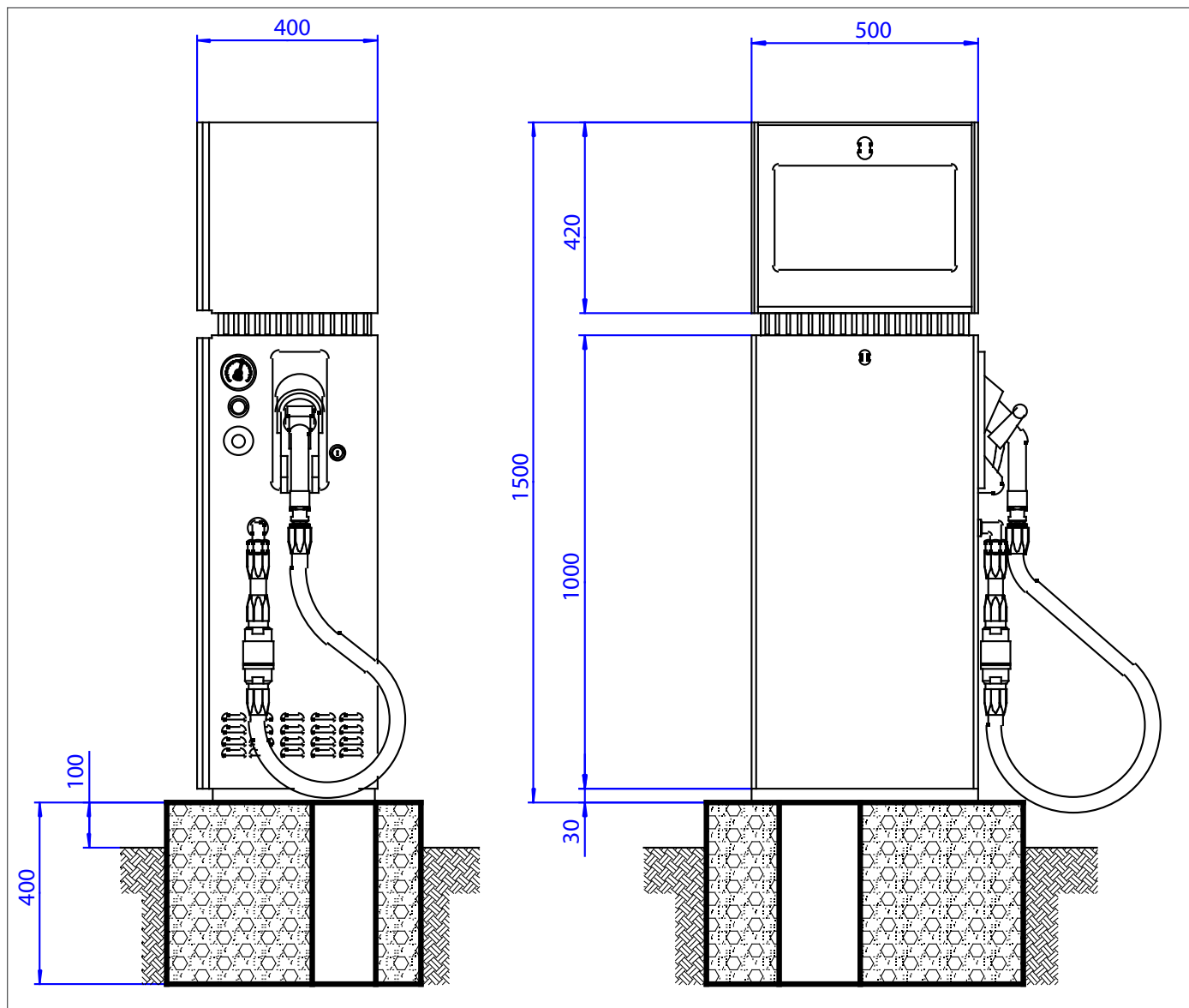
Dimensional drawing of LPG-dispenser type EDS-120
