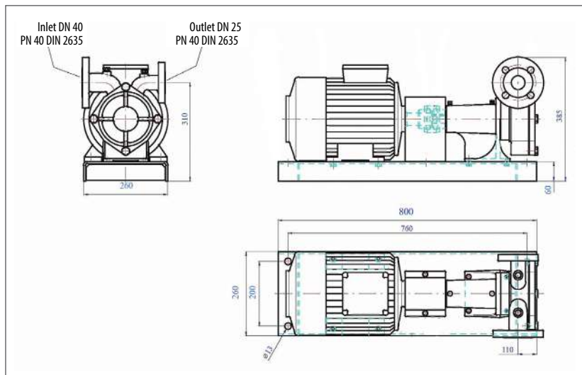
Dimensional drawing of the pump unit EDS-Corken FD-150
