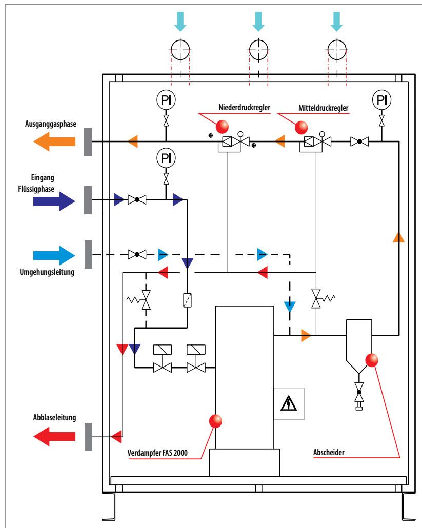
Typical diagram of vaporizer unit EDS 2000
