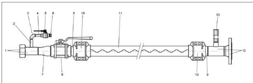
EDS 25 027 LPG-filling hose DN 50 in full hose system
