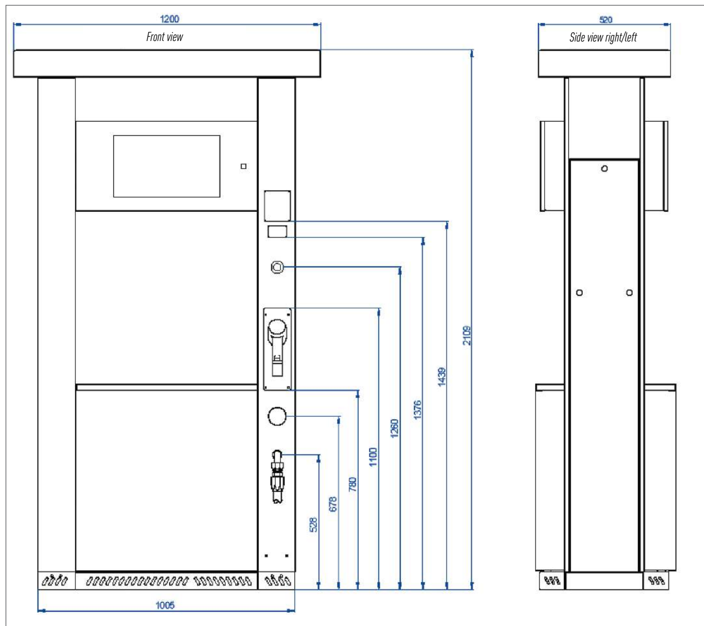
Dimensional drawing of electronic LPG-dispenser Type EDS-220/EDS-230
