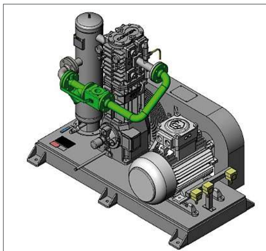
Compressor unit Type EDS
